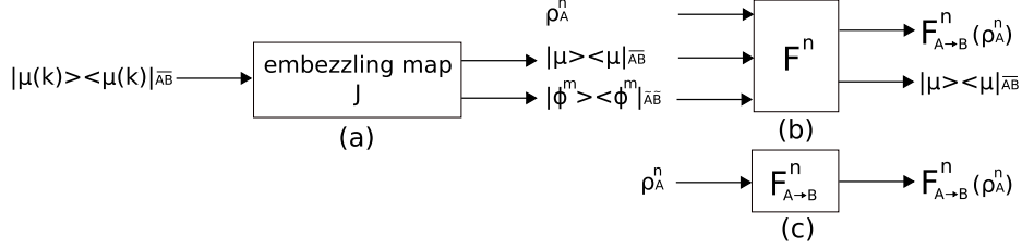
Fig. 1. (a) \mathcal{J} is the map that embezzles m maximally entangled states |\Phi^m\rangle\langle\Phi^m|_{\tilde{A}\tilde{B}} out of |\mu\rangle\langle\mu|_{AB} . These maximally entangled states are then used for a symmetrization step. (b) The whole protocol \mathcal{F}_{A\rightarrow B}^n (that should simulate \mathcal{E}_{A\rightarrow B}^{\otimes n} ) a priori takes \rho_A^n \otimes |\mu\rangle\langle\mu|_{AB} \otimes |\Phi^m\rangle\langle\Phi^m|_{\tilde{A}\tilde{B}} as an input. But since this input is constant on all registers except for A , we can think of the map as in (c), namely as a CPTP map \mathcal{F}_{A\rightarrow B}^n which only takes the input \rho_A^n .
